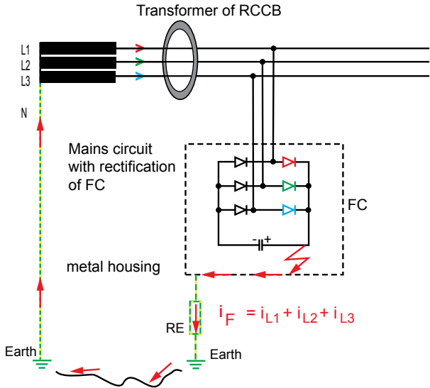
Fig. 10: Effect of an insulation fault at the intermediate circuit capacitor with six-pulse bridge connection
