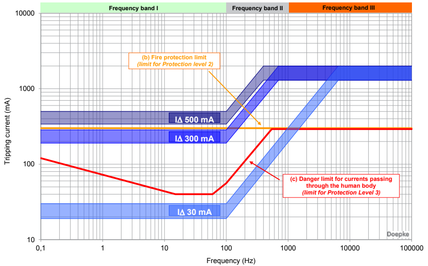
Fig. 15: Frequency responses of the tripping current for the residual current circuit-breaker DFS 4 B SK in relation to the hazard limits for personal and fire protection
