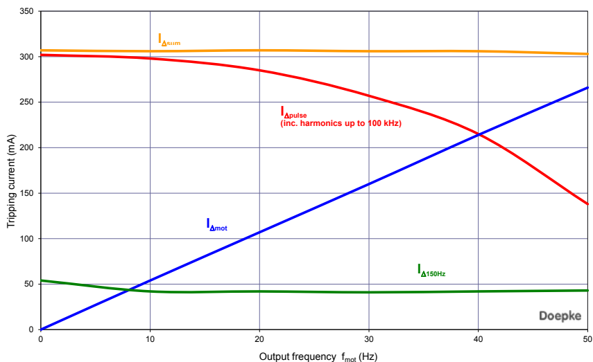
Fig. 13: Residual current components of various frequencies at the output of a three-phase operated frequency converter at a clock frequency of 8 kHz and a fault loop resistance of 780 ohm
