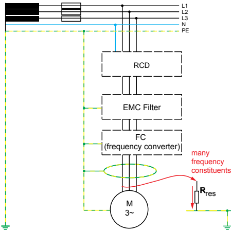
Fig. 6: Residual current with frequency mix
