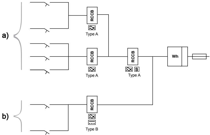
Fig. 9: Division of electric circuits in systems with electronic equipment (source: DIN VDE 0160 / EN 50178, HD 60364-5-53 Annex A Figure A.2)
