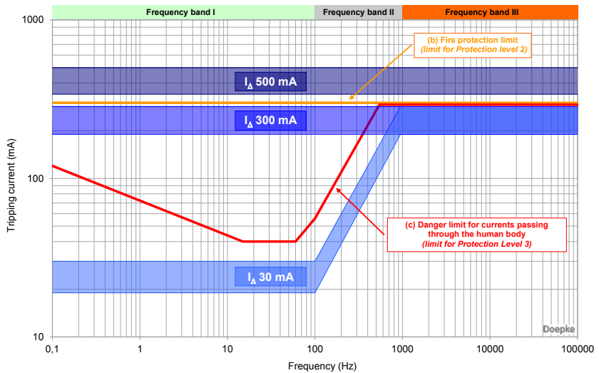
Fig. 14: Frequency responses of the tripping current for the residual current circuit-breaker DFS 4 B NK in relation to the hazard limits for personal and fire protection
