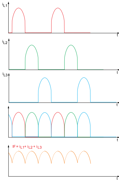
Fig. 11: Representation of individual conductor currents
