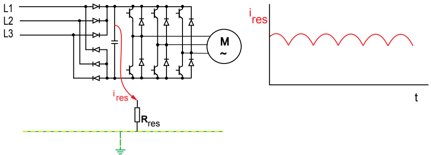
Fig. 1: Production of an almost smooth DC residual current (simplified representation of a frequency converter with B6 bridge rectifier, intermediate circuit capacitor, output level and motor)
