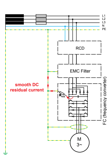
Fig. 5: DC residual current
