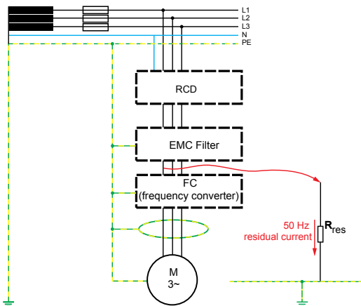
Fig. 4: Residual current of 50 Hz
