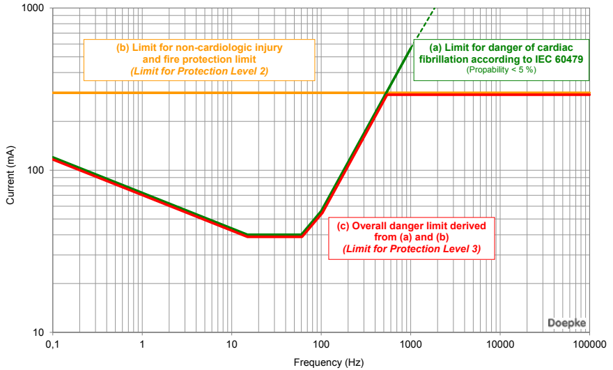
Fig. 12: Hazard limit values for various effects of current passing through the human body
