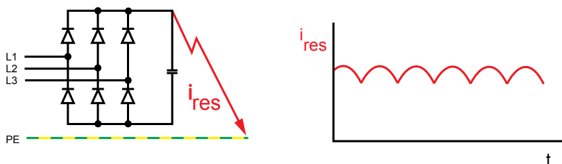
Fig. 8: Six-pulse bridge connection (three-phase AC bridge connection)
