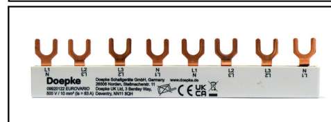
four pole busbar
